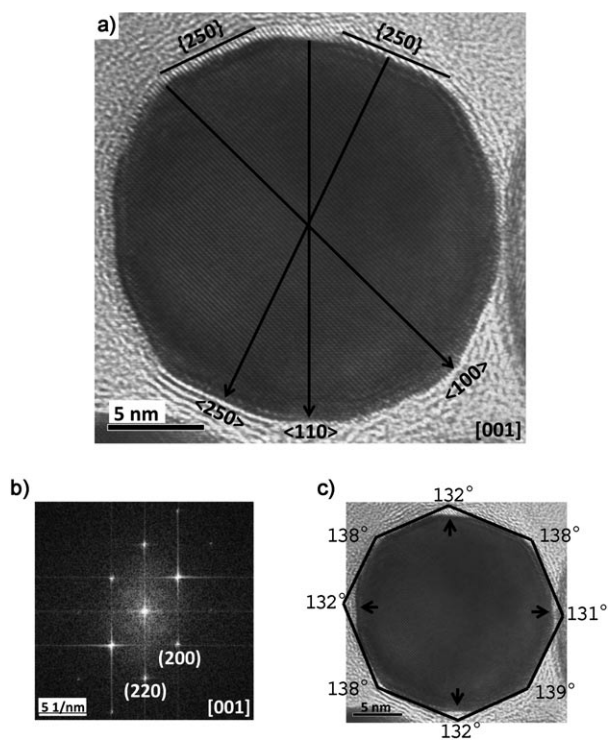
Figure 1. a) HRTEM image of a standing gold nanorod, showing the main crystallographic directions and the indexes of the facets. b) Corresponding FFT spot pattern demonstrating the [001] zone axis. c) Measured angles between lateral facets showing the approximate alternation of angles; the arrows point to \langle 110 \rangle -type directions, where small bevels can be seen.
