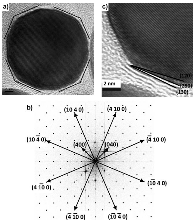
Figure 2. Method used to calculate the index of the side facets. Lines drawn in (a) are perpendiculars to the (4 10 0) direction vectors drawn in (b). c) Comparison of the agreement achieved with {120}-, {130}-, and {250}-type facets.
